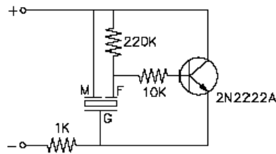
Figure 1. Feedback Circuit
